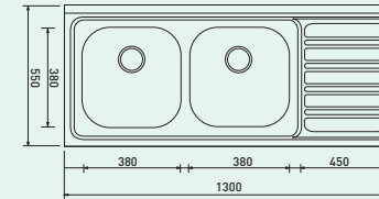
DOUBLE SINK BOWL SD 1300(L/R)
