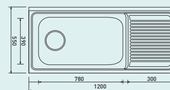
JUMBO SINK BOWL JS 1200(L/R)
