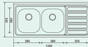
DOUBLE SINK BOWL SD 1200(L/R)
