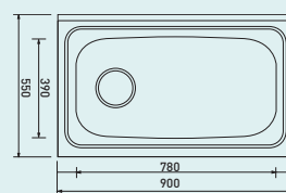
JUMBO SINK BOWL JS 900
