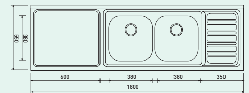
DOUBLE SINK BOWL LSD 1800
