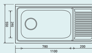
JUMBO SINK BOWL JS 1100(L/R)
