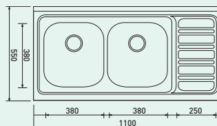
DOUBLE SINK BOWL SD 1100(L/R)
