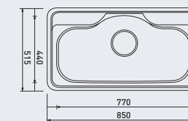
INSET(UNDER) BOWL DJIS 850
