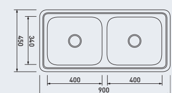
INSET(UNDER) BOWL ISD 900
