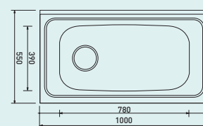
JUMBO SINK BOWL JS 1000
