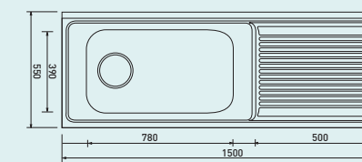
JUMBO SINK BOWL JS 1500(L/R)
