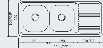
INSET(UNDER) BOWL ISD 1100/1310
