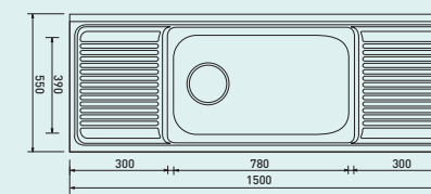
JUMBO SINK BOWL JSC 1500
