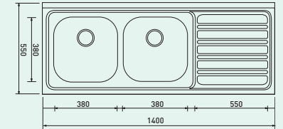
DOUBLE SINK BOWL SD 1400(L/R)
