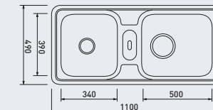
INSET(UNDER) BOWL ISB 1100(L/R)
