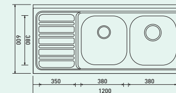
DOUBLE SINK BOWL XSD 1200
