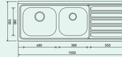
DOUBLE SINK BOWL LSD 1500(L/R)
