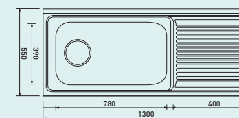
JUMBO SINK BOWL JS 1300(L/R)
