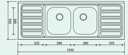
DOUBLE SINK BOWL SDC 1500
