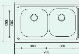
DOUBLE SINK BOWL SD 900
