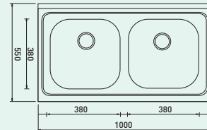
DOUBLE SINK BOWL SD 1000
