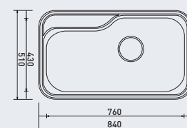
INSET(UNDER) BOWL NJIS 840(L/R)
