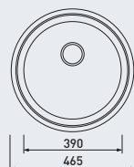
INSET(UNDER) BOWL RB 46
