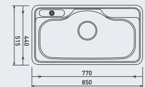
INSET(UNDER) BOWL DJIS 850P
